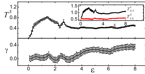
FIG. 2 (color online). Same as Fig. 1 but for a Lorenz system driven by a Rössler system. Error bars indicate standard deviations from 100 realizations of the systems, with initial conditions chosen randomly close to the attractors of both systems for each realization.
